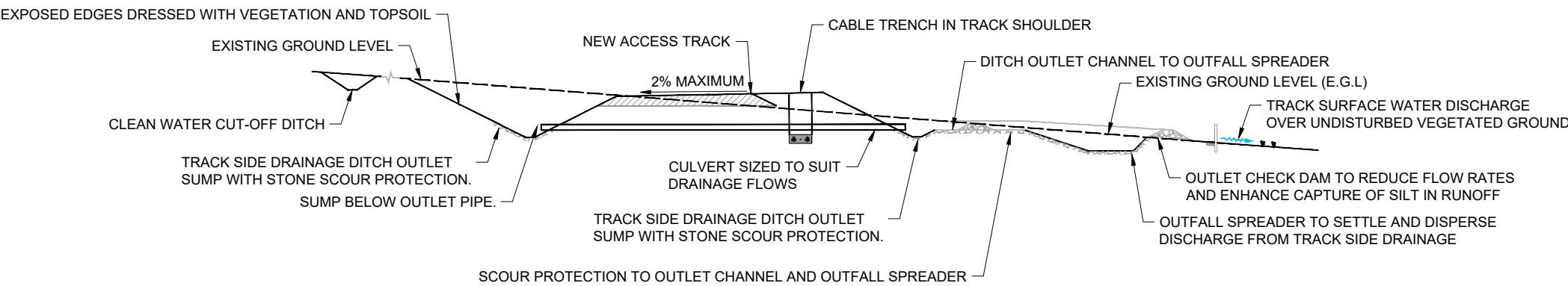
TYPICAL ACCESS TRACK DRAINAGE - SECTION A - A
