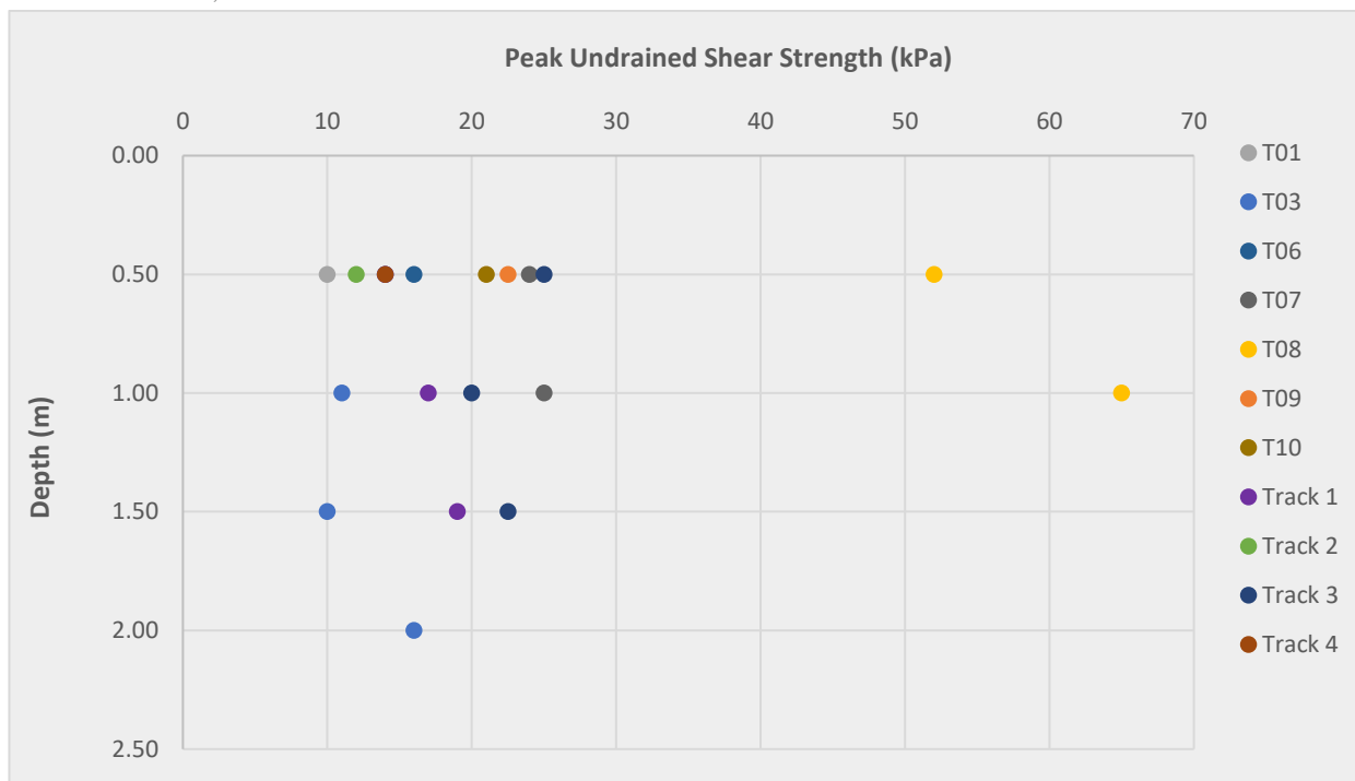
Figure 3.2: Peak Undrained Shear Strength (kPa) against Depth (mbgl) across the areas of key infrastructure at the Proposed Development.
