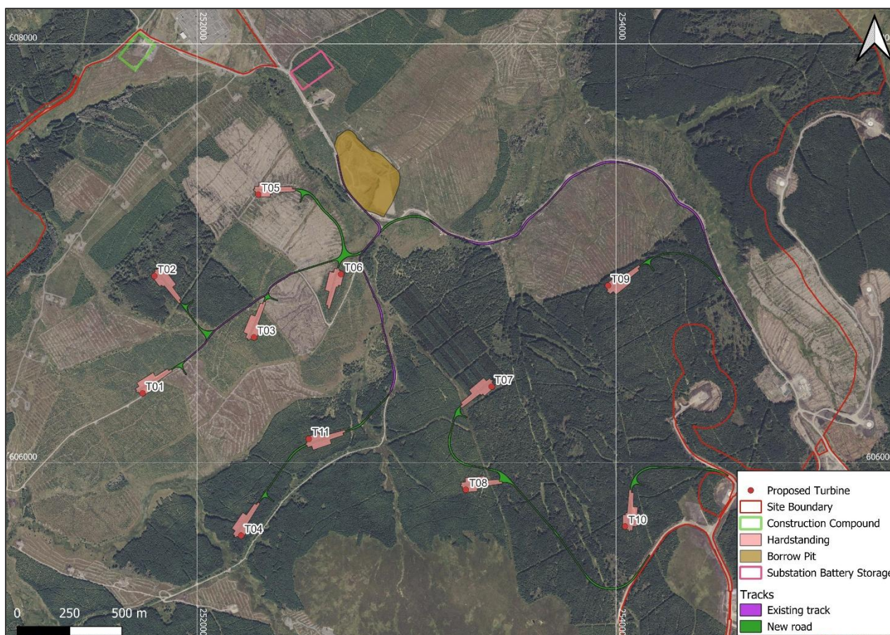
Figure 1.2: Amended Site layout with approximate Turbine Locations and associated infrastructure
