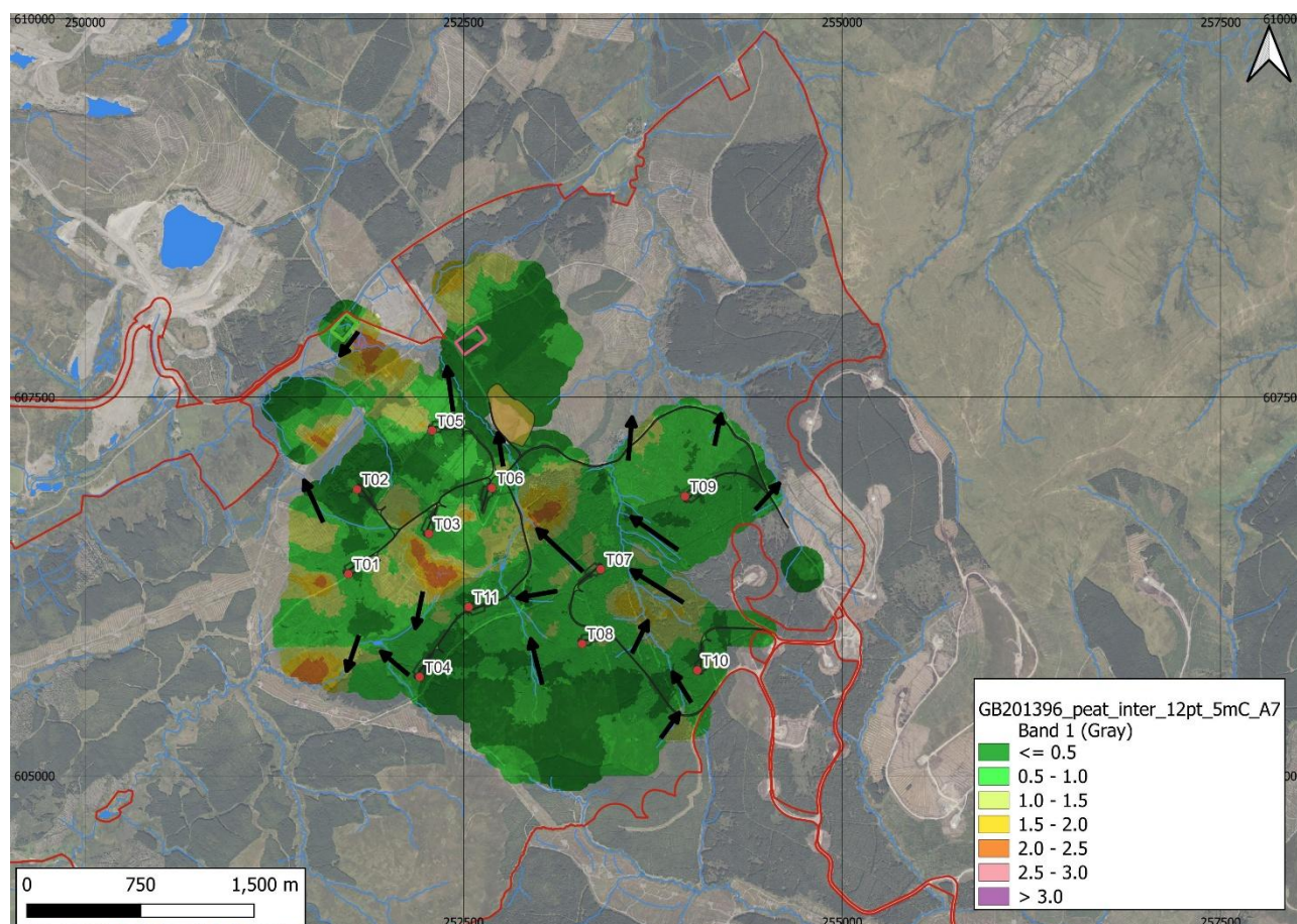
Figure 6.1: Preliminary peat slide pathways (black arrows) and indicative peat depth.
