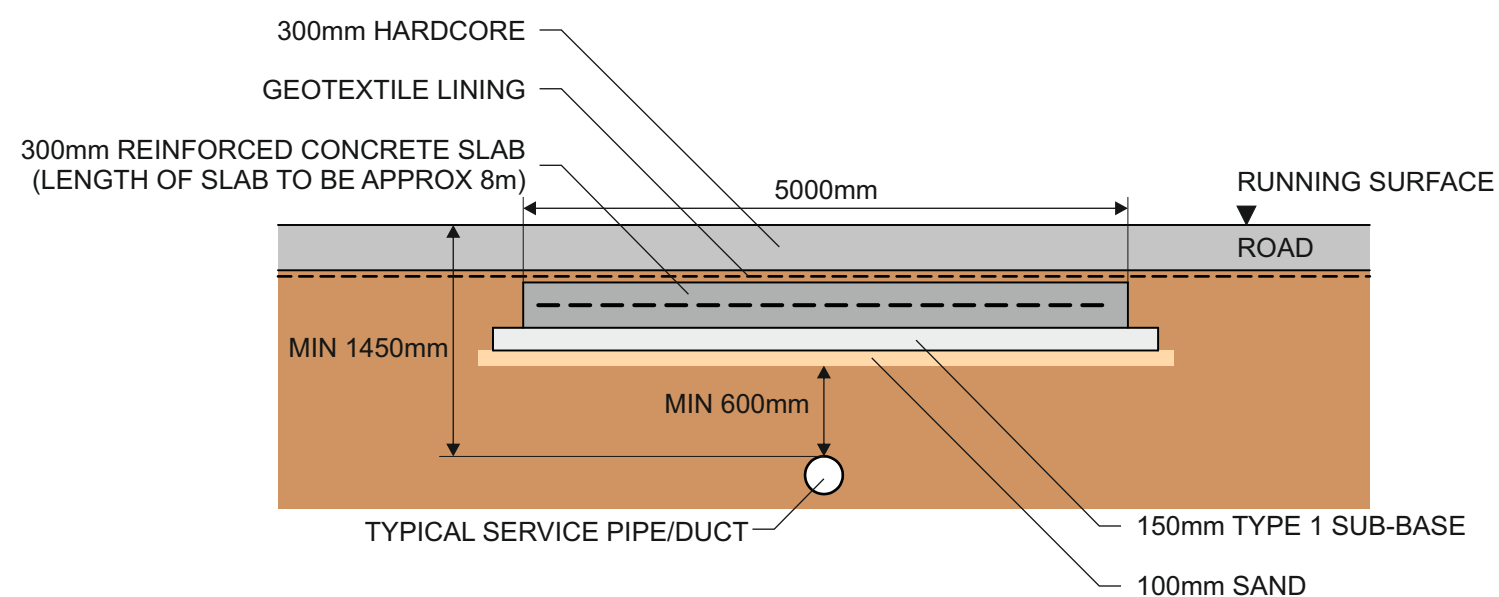
INDICATIVE PROTECTION TO SERVICES
