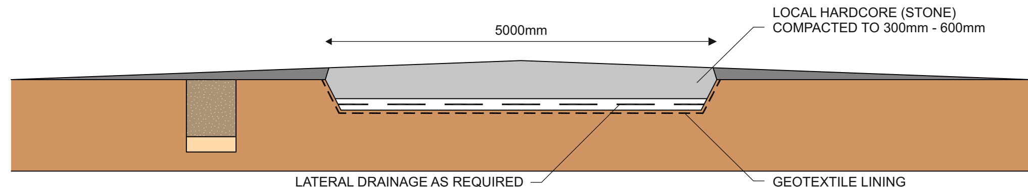
TRACKS CLOSE TO ROCKHEAD
