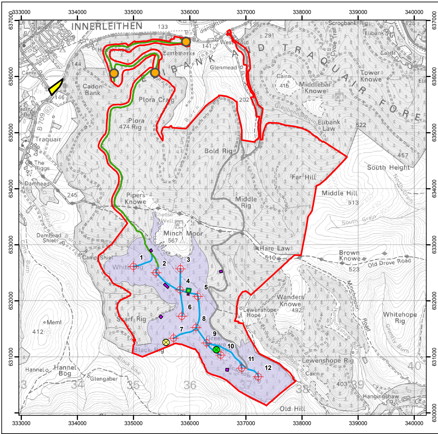
FIGURE 1 Site Layout
